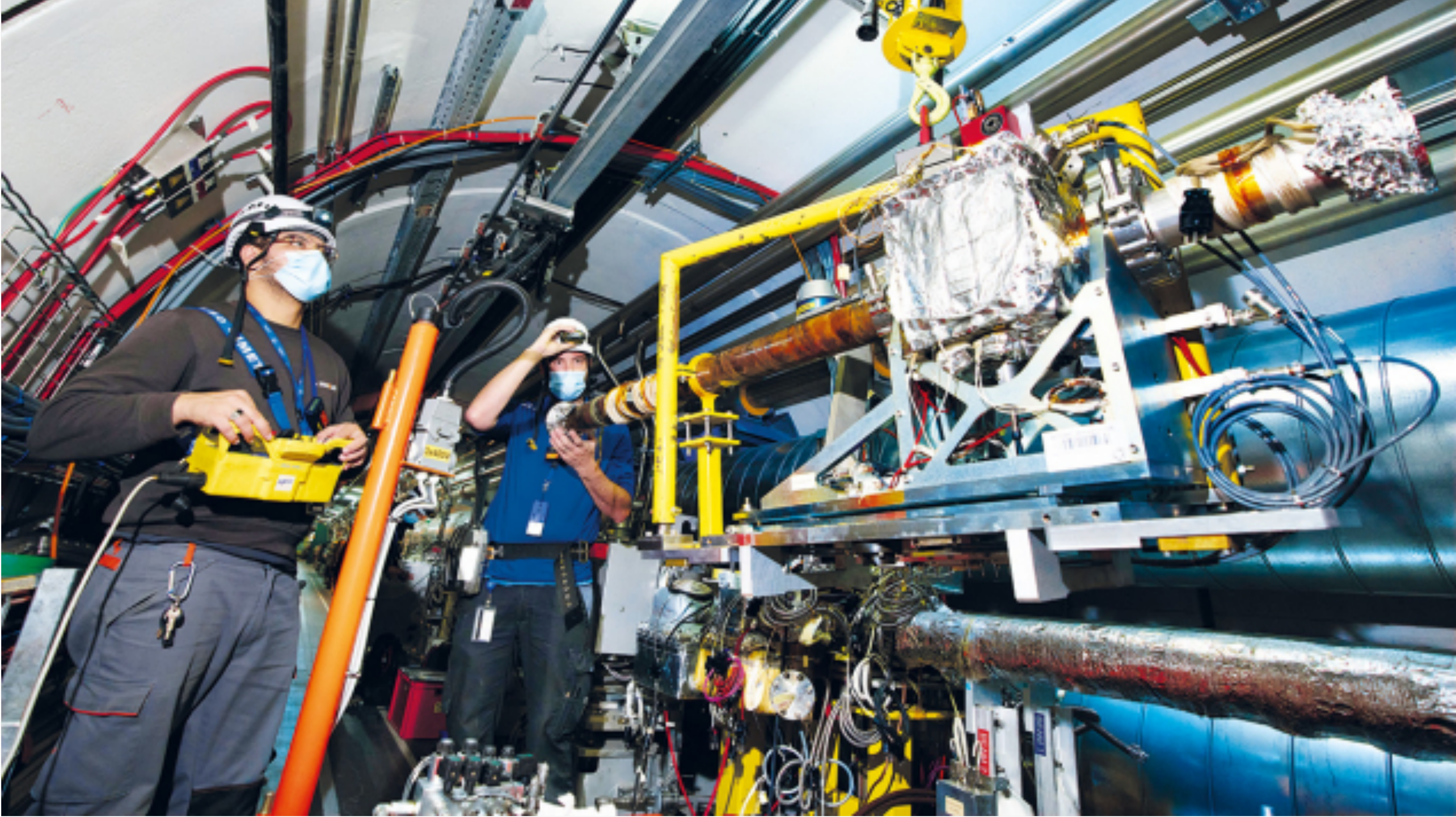
Heavy-ion collimation A crystal collimator is installed at the LHC, where it is used to deflect halo particles onto an absorber located roughly 90 metres downstream. Credit: JM Ordan/CERN-PHOTO-202111-085-3
