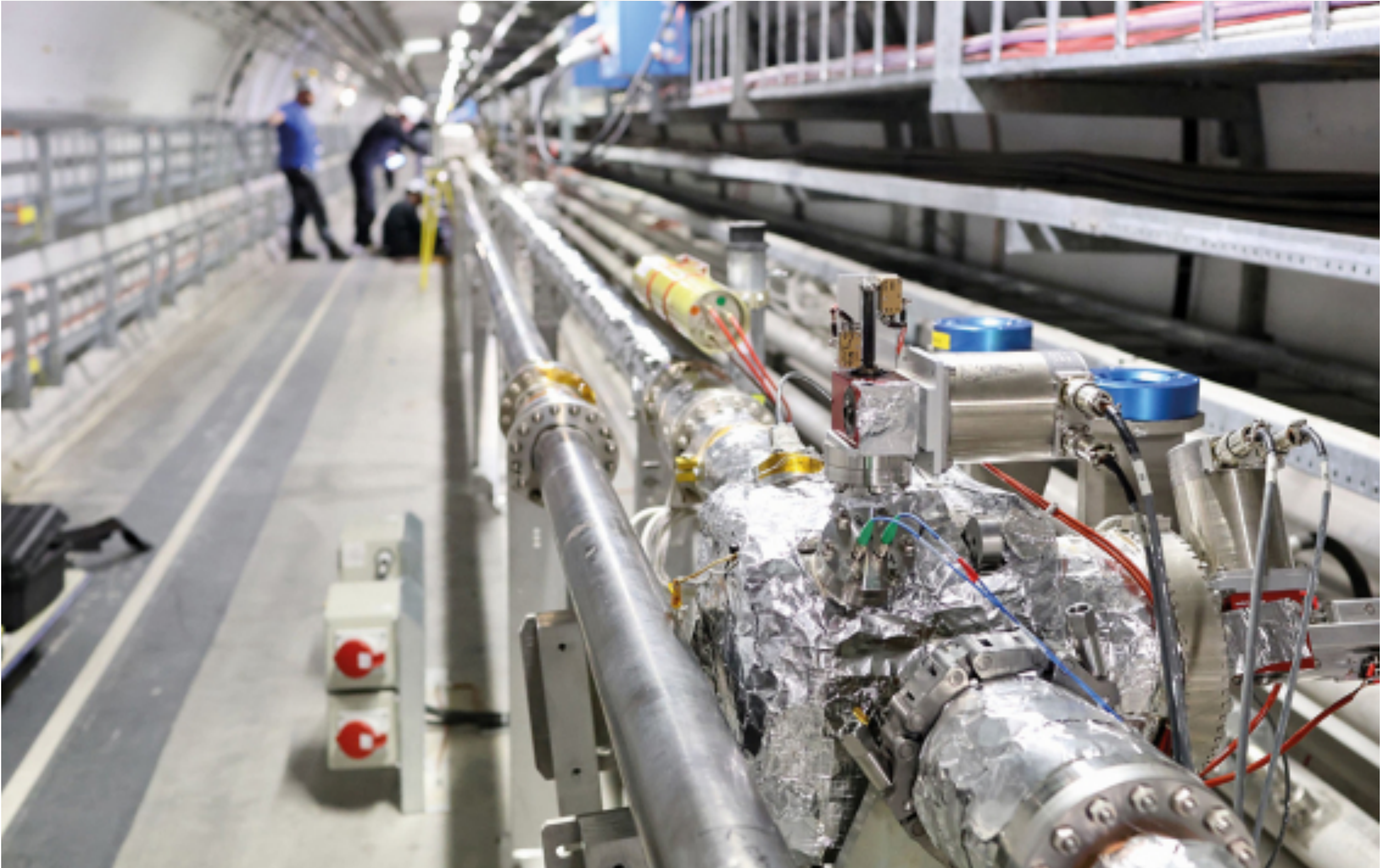
action The first bent crystal of the TWOCRIST experiment extracts protons from the halo of the circulating LHC beam and directs them onto a second bent crystal 120 metres downstream, leading to the first demonstration of double channelling of TeV particles last year. Credit: S Redaelli/CERN-PHOTO-202503-098-2
