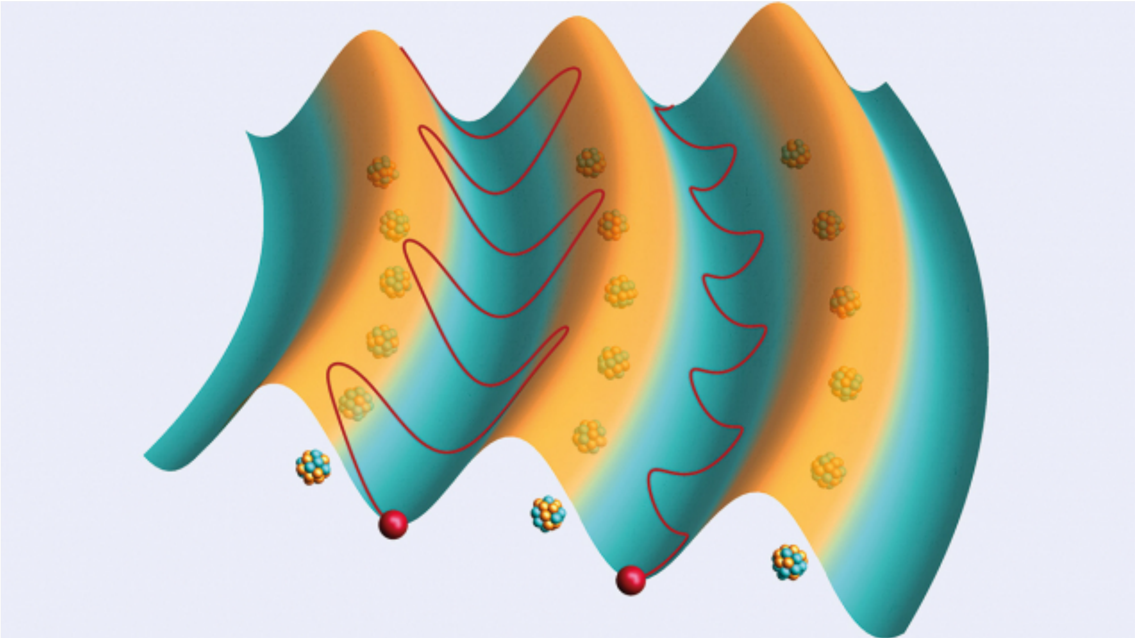
Guided paths Positively charged particles (red) can be "channelled" along the trough of the electrostatic potential (shaded surface) between planes of nuclei in a bent crystal, achieving a far stronger curvature than conventional magnets. In this artist's impression, length scales have been adjusted for clarity. Credit: D De Biasio
