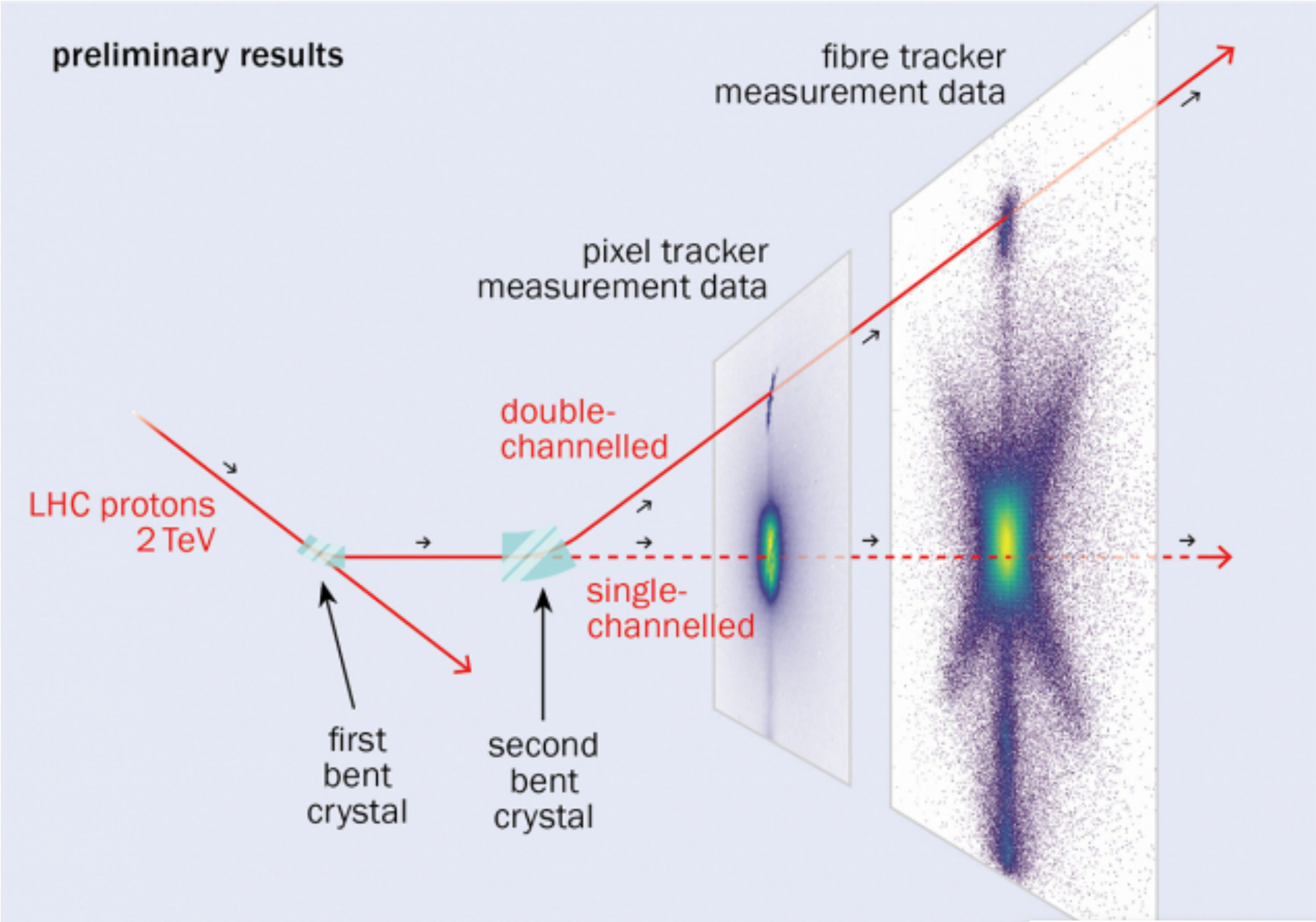
Double channelling in TWOCRIST. A 4 mm splitting crystal deflects protons by about 50 microradians, followed 120 metres downstream by a 5 mm fixed tungsten target and a 7 cm-long precession crystal with a bending angle of 7 milliradians. Downstream of the crystals, movable vacuum chambers and a fibre tracker provided by the ATLAS-ALFA collaboration. Credit: TWOCRIST/J V Dos Santos
